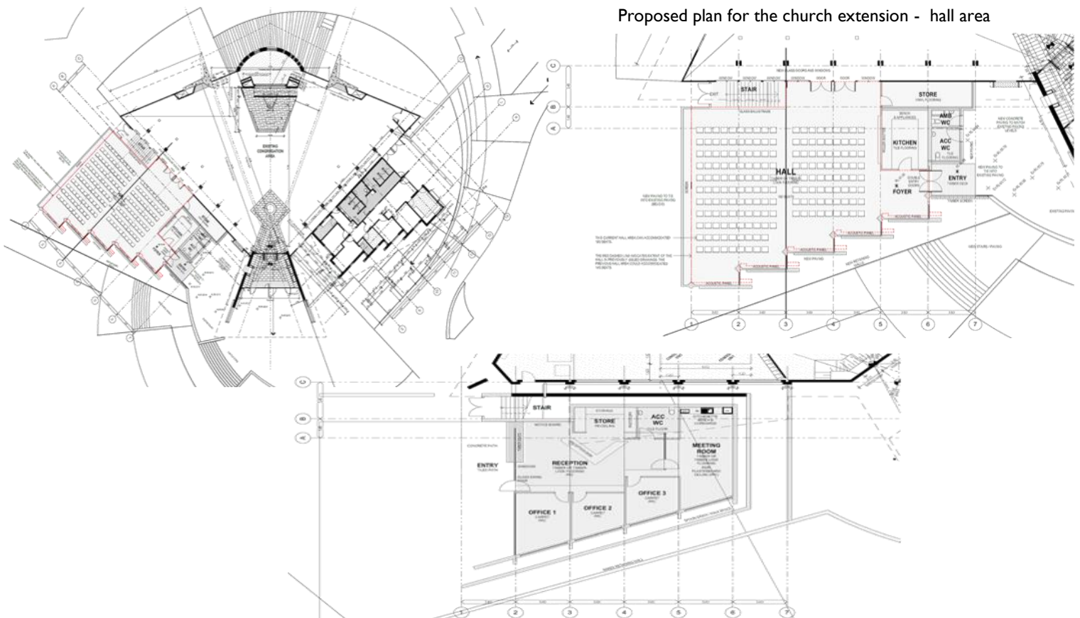
HALL EXTENSION - SOUTH ENTRY
